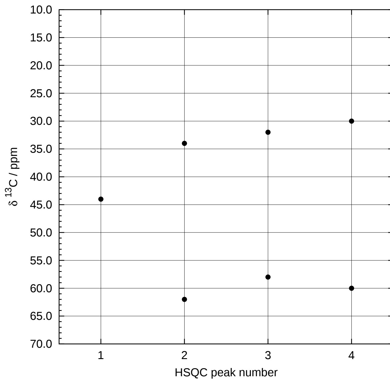
CBCA(CO)NH Spectrum 1
