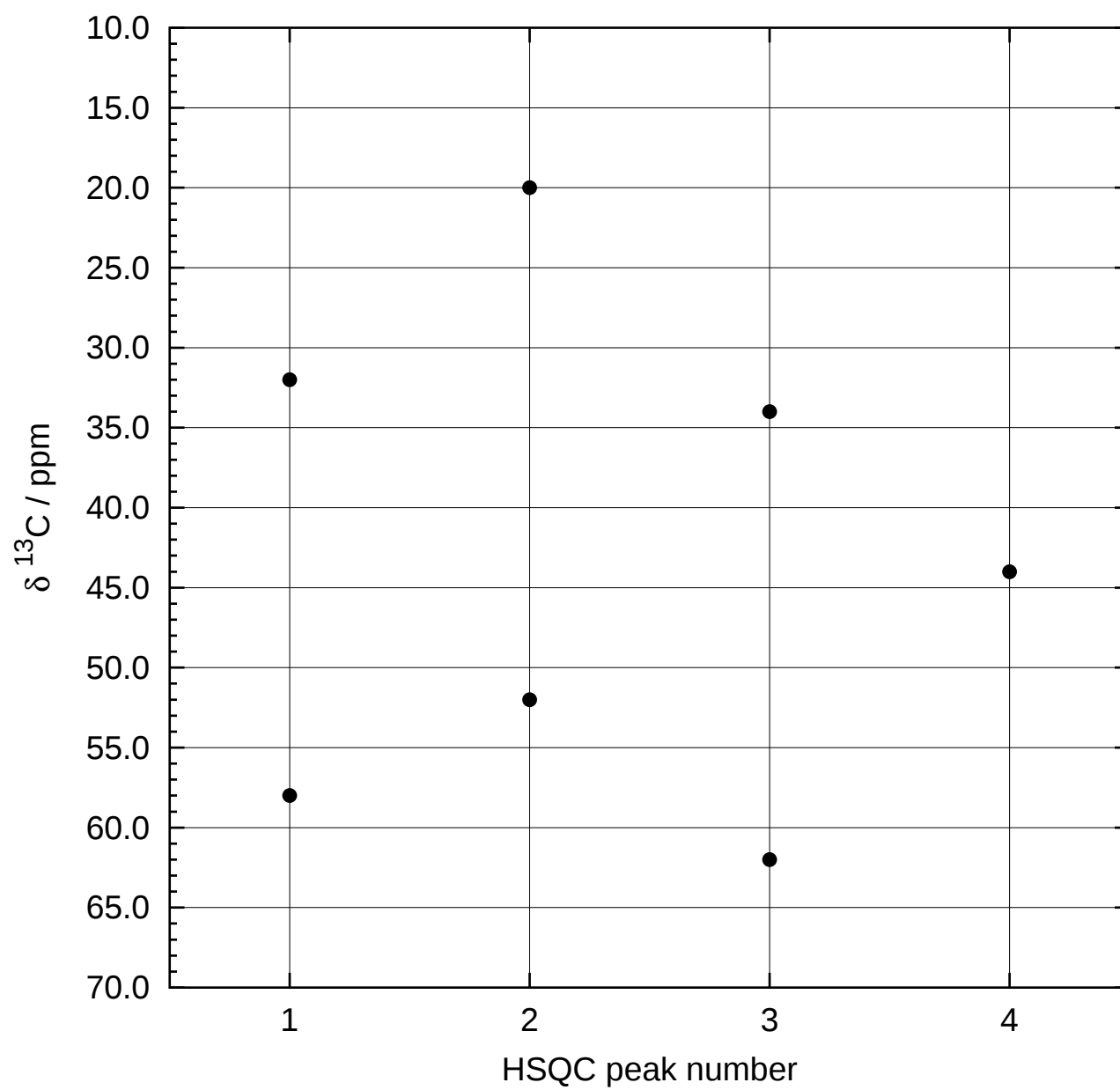
HNCACB Spectrum 1
