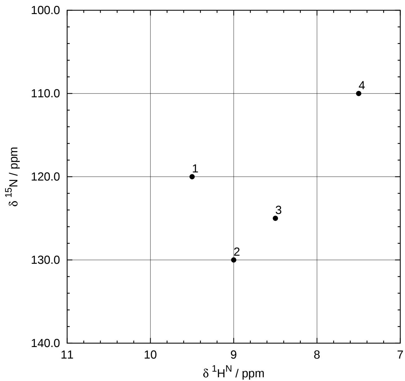
HSQC Spectrum 1
